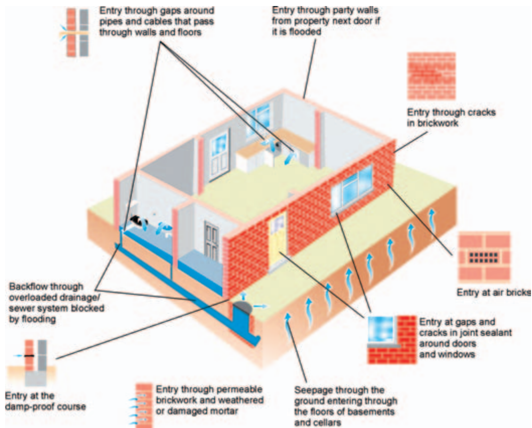
Figure 2.6 Potential Routes for Entry of Flood Water into a Dwelling (courtesy of CIRIA, after CIRIA 2003)
