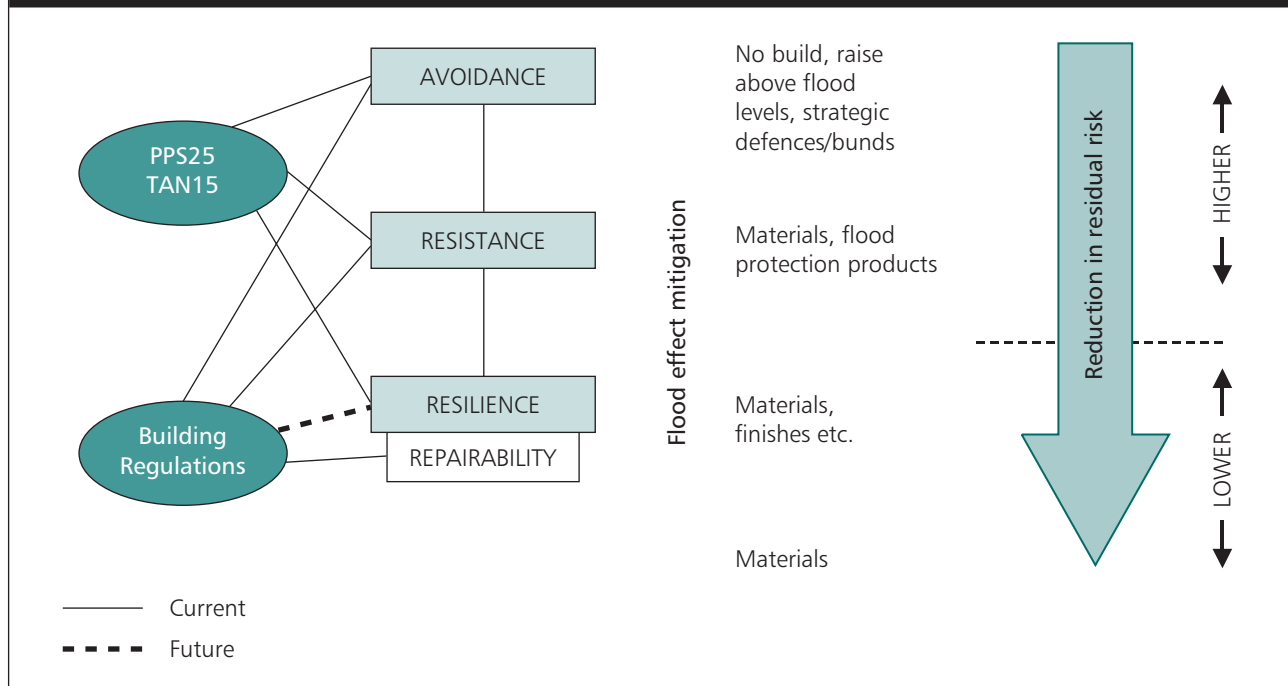
Figure 2.3 Flood risk management hierarchy
