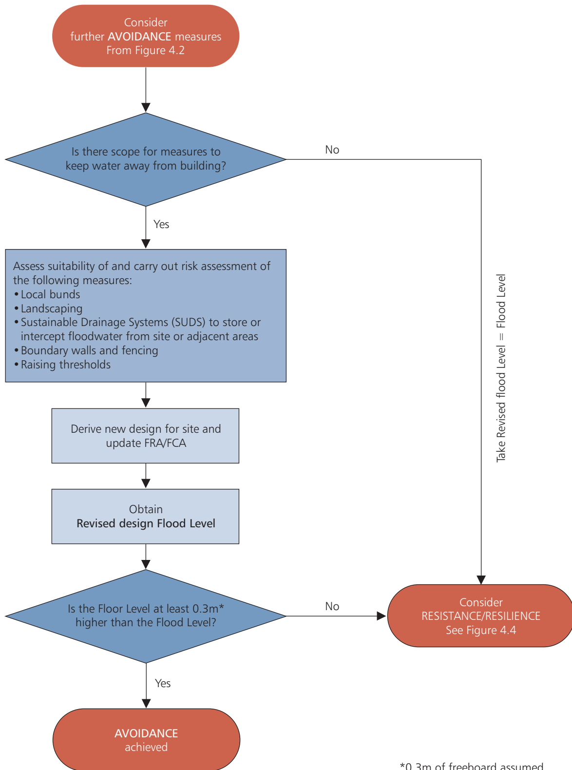
Figure 4.3 Design strategies; decision flowchart – Avoidance (2)
