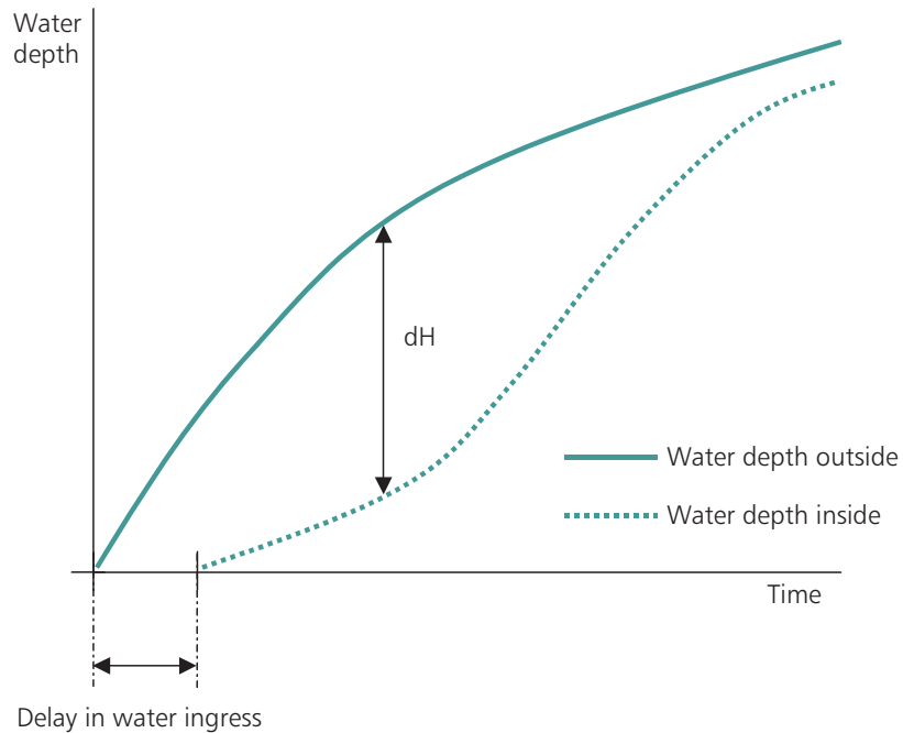
Figure 2.5 Conceptual illustration of flood water depths outside and inside a building
