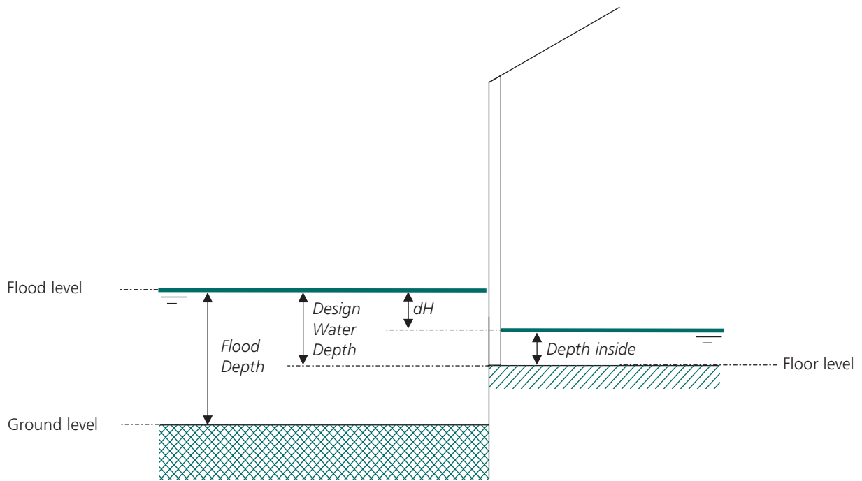
Figure 2.4 Definitions of flood depths
