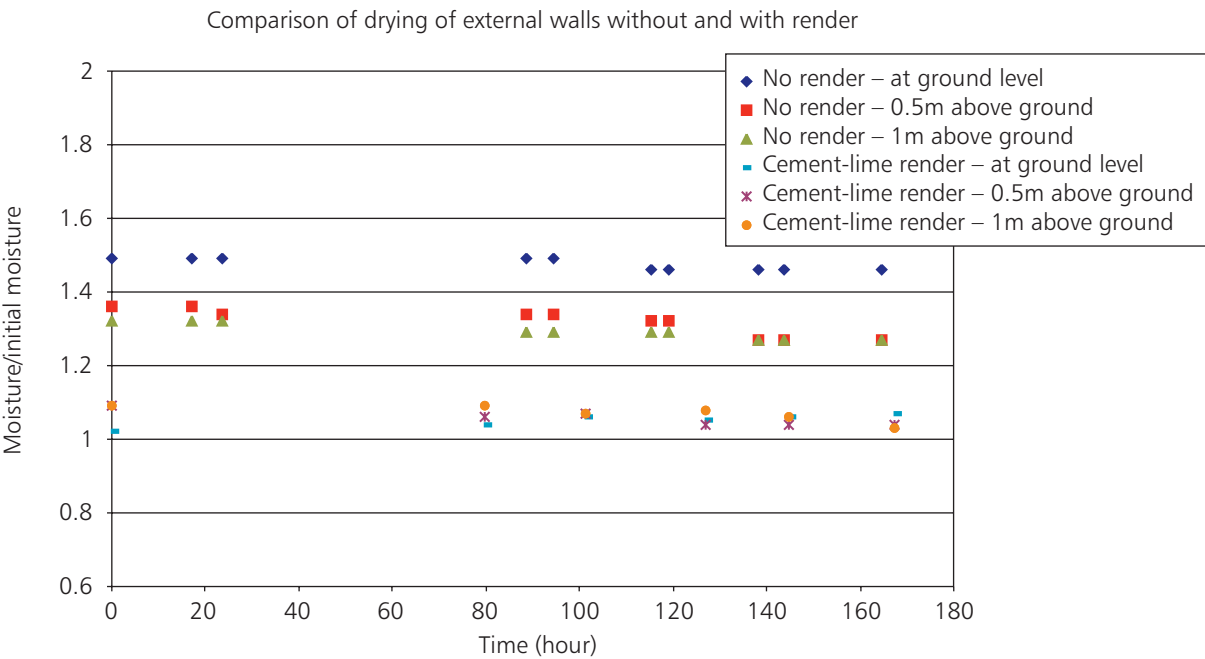
Figure 7.3 Example of effect of render on surface drying of external brick wall (reduction in surface moisture; 1.0 equivalent to pre-flood condition)
