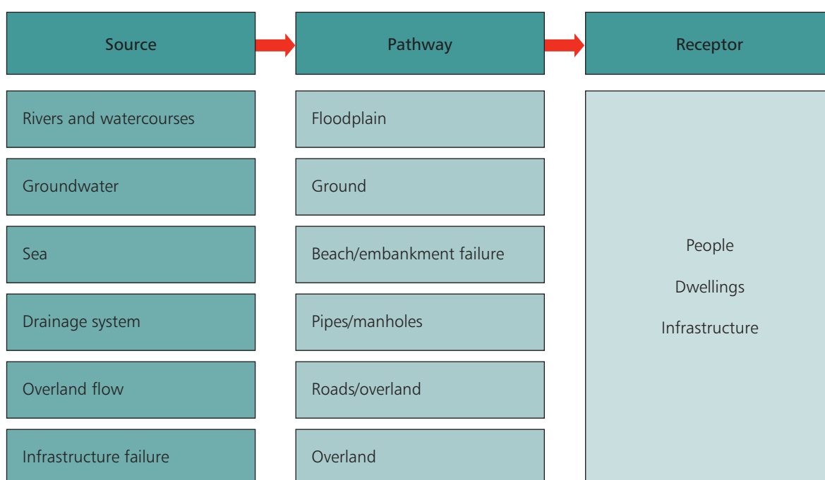
Figure 2.1 Flood risk management – the concept of source-pathway-receptor
