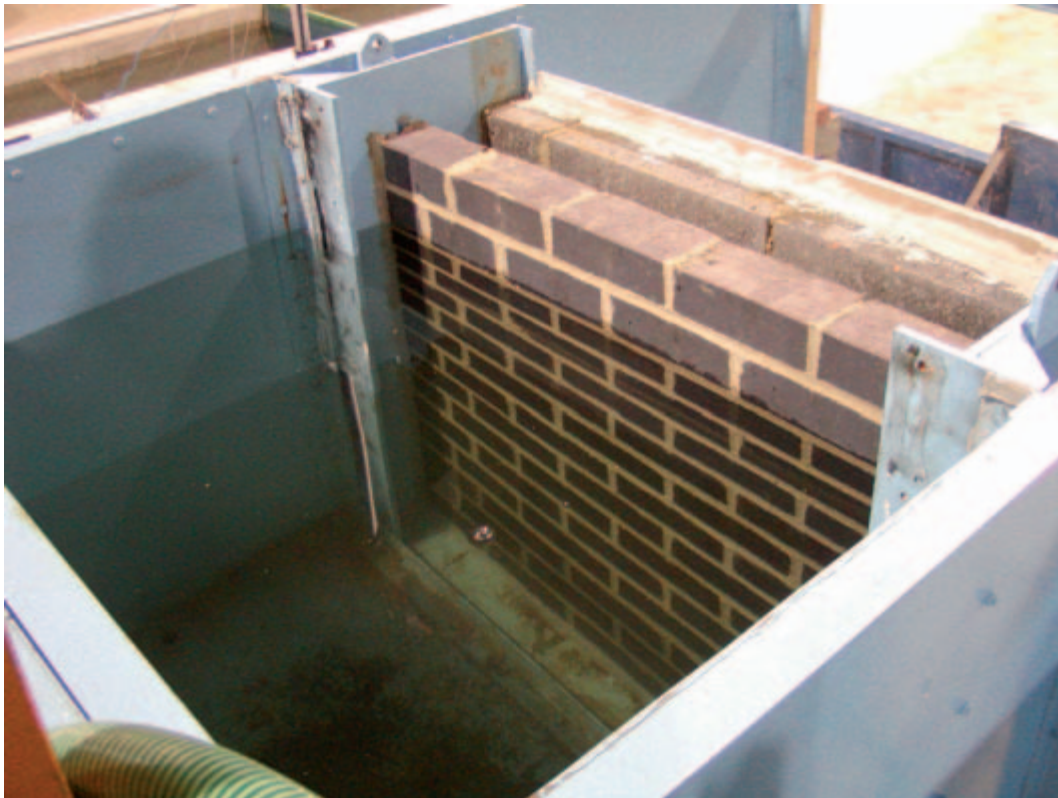
Figure 7.5 Testing a cavity masonry wall
