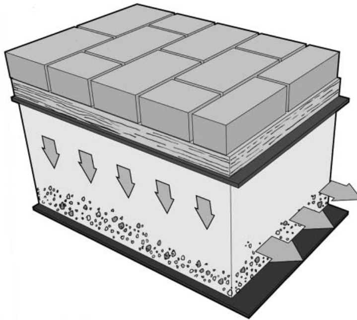
Figure 3.10: Permeable pavement – typical vertical section. Source: adapted from Butler and Davies 2011.
