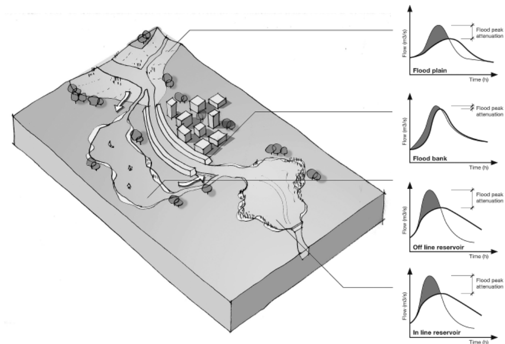
Figure 3.6 Attenuation of conveyance and storage devices within a catchment, Source: Baca Architects
