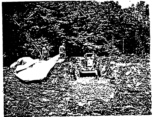
6. This anoxic limestone drain, which is being built with the help of the National Guard, will add alkalinity to acidic drainage from an abandoned coal mine before wetland treatment.
