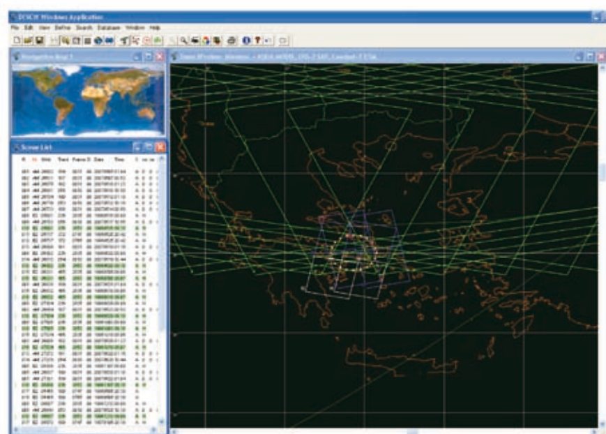
Figure 2.20. View of DESCW user interface.
