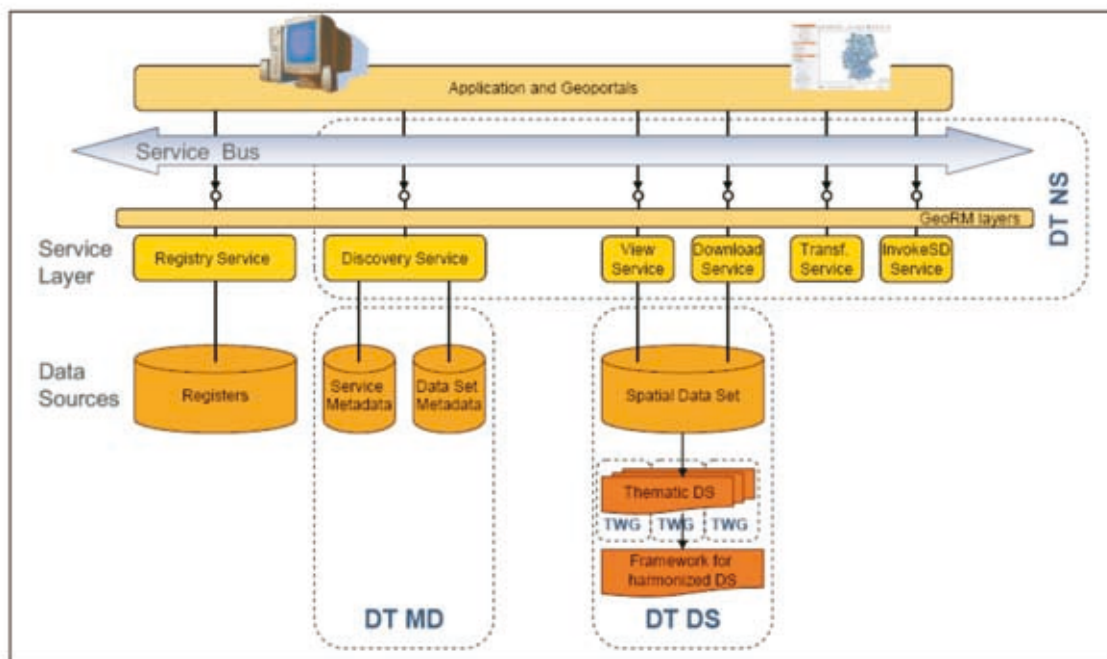
Figure 1.10. INSPIRE Technical Architecture Overview.
