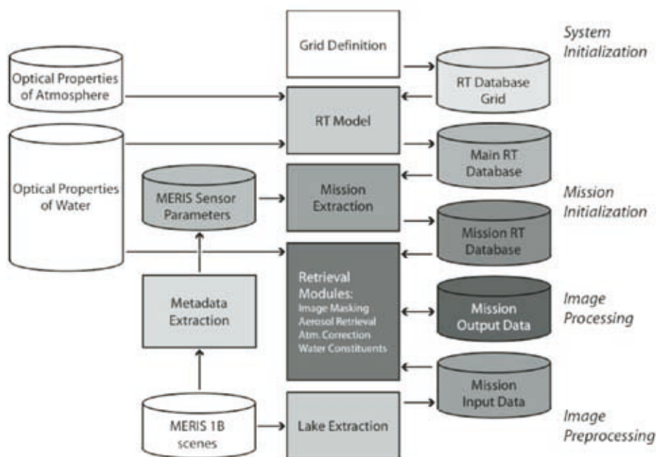
Figure 3.43. Schematic Diagram of MIP Inland Water Processor.
