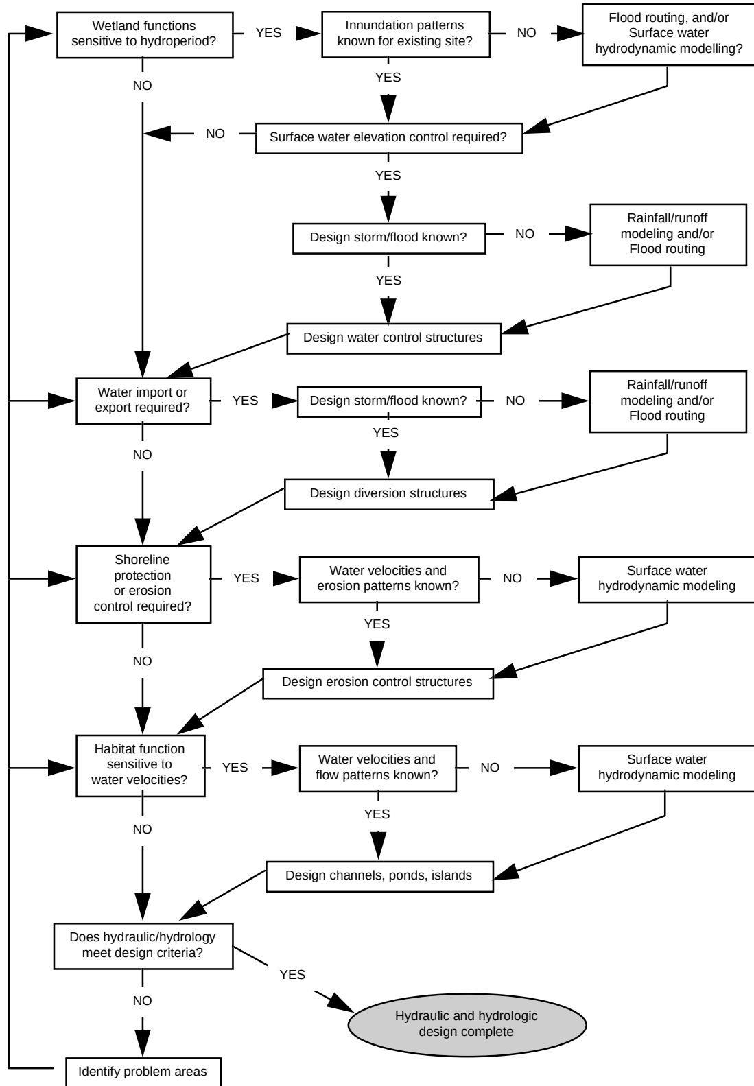
Figure 5-2. Hydrologic and hydraulic design process for wetlands.
