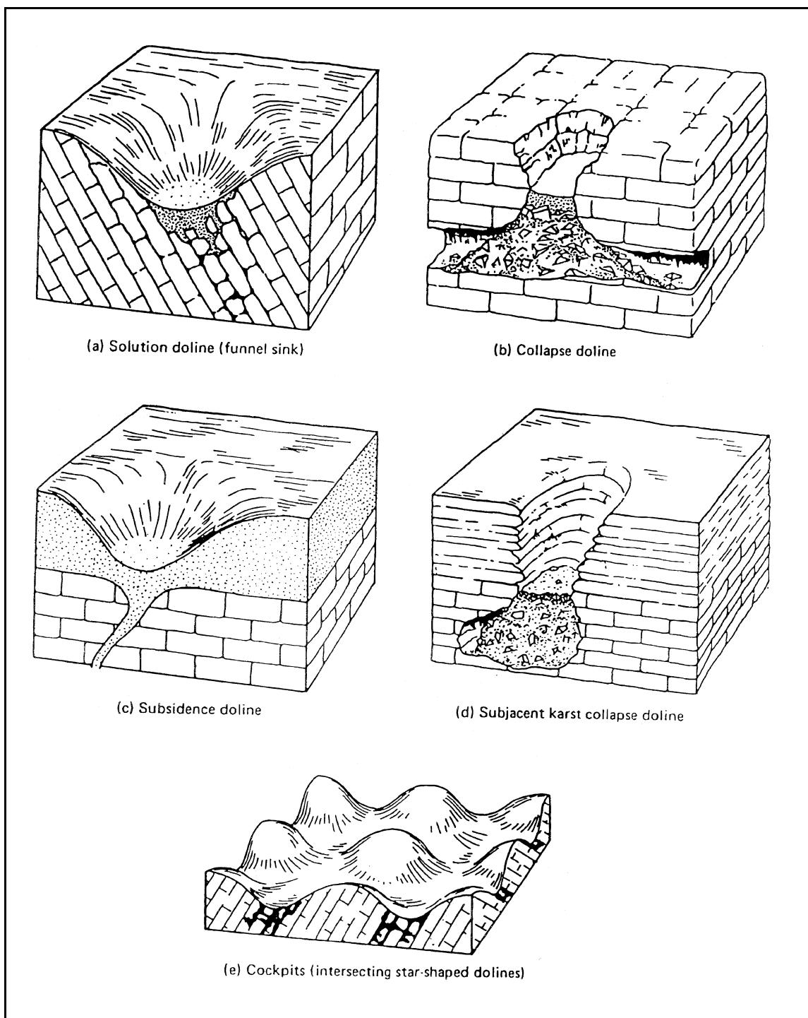
Figure 3-7. Block diagram of karst features associated with the five types of dolines (after Jennings 1985).
