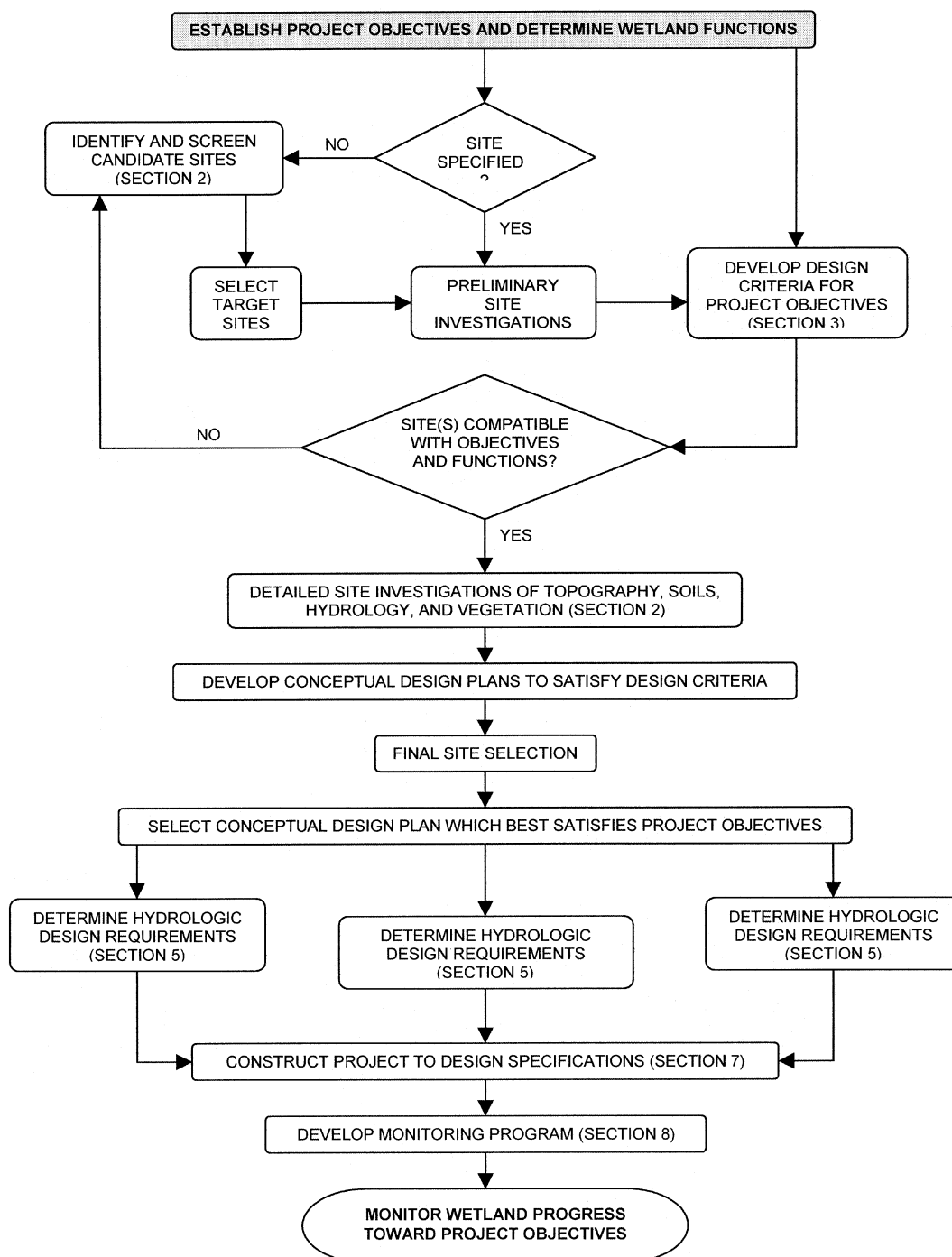
Figure 1-1. Decision sequence for wetlands restoration and creation projects.
