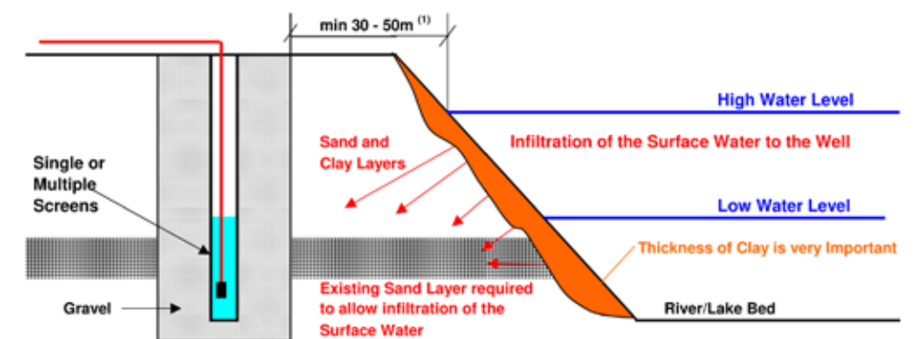
Figure 3: Typical design of RBI
