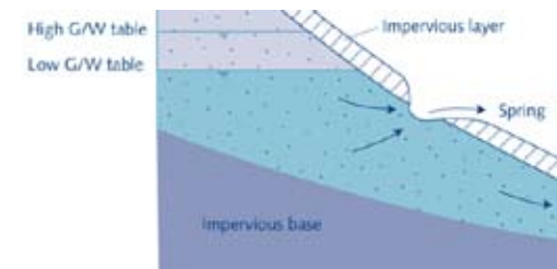
Figure 1: Example of an artesian depression spring (Wijk-Sijbesma et al, 2002).
