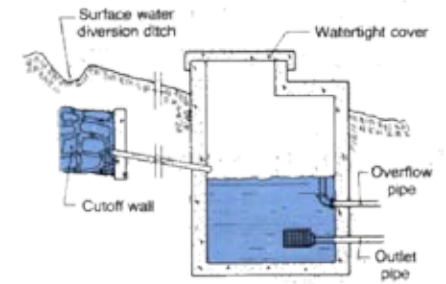
Figure 2: Cut-away view of a concentrated spring (Jennings, 1996)
