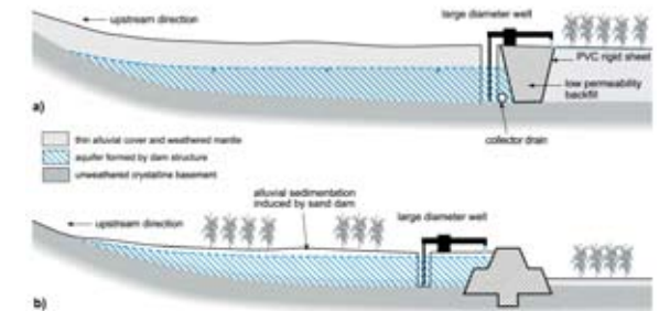
Figure 1: Typical design of subsurface dam (Source: GWMATE)
