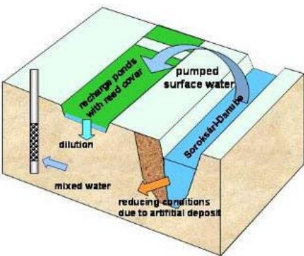
Figure 4: RBI with recharge ponds
