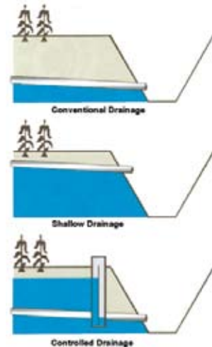
Figure 1: Various piped drainage systems
