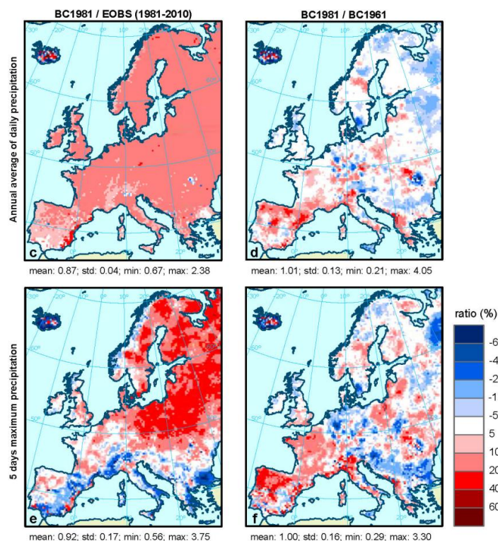
Figure III-3: Assessment of bias corrected daily precipitation in the period 1981-2010 for the climate simulation METO-HadRM3Q0-HadCM3Q0. Left column shows the ratio between bias corrected precipitation and observations from the E-OBS data set. The right column shows the ratio between the current period (1981-2010) and the previous bias correction period (1961-1990). The first row shows the annual daily average precipitation whereas the second row shows 5-days maximum precipitation.
