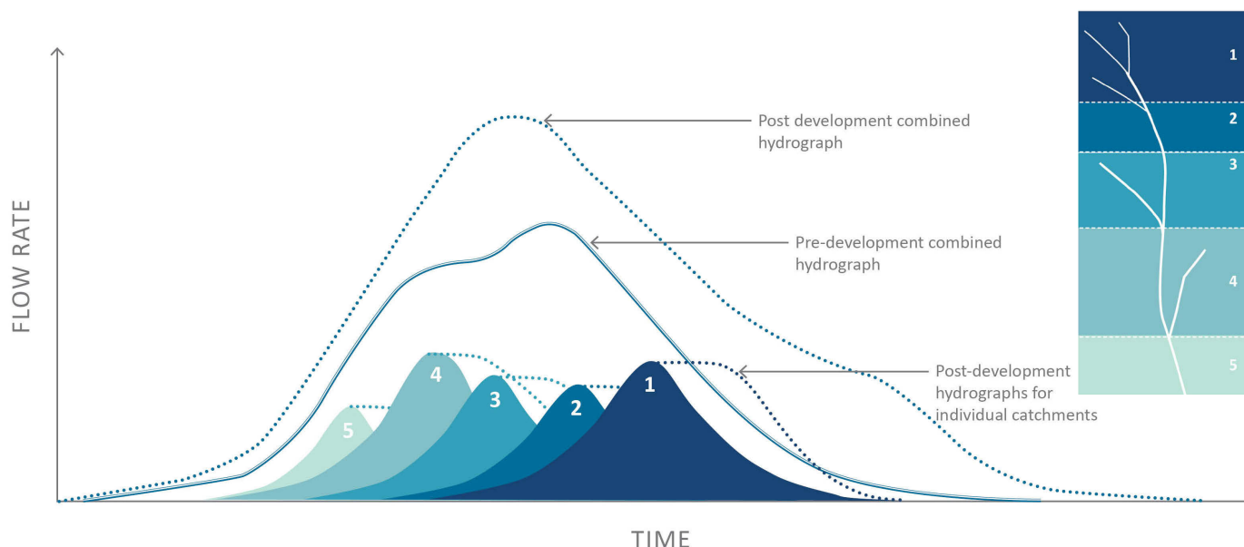
Figure 9: Superposition of peak flows from multiple catchments with extended detention (adapted from Shaver, 2000)
