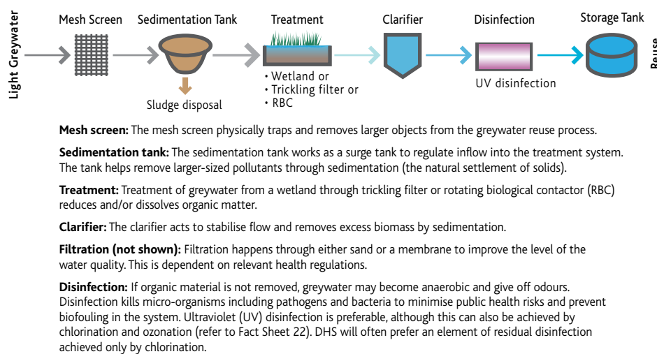
Figure 8. Typical treatment train for a greywater reuse system
