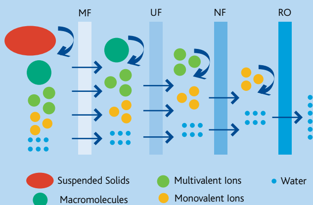
Figure 1 Types of membranes and membrane selectivity (reproduced from Bhattacharjee et al (1999))
