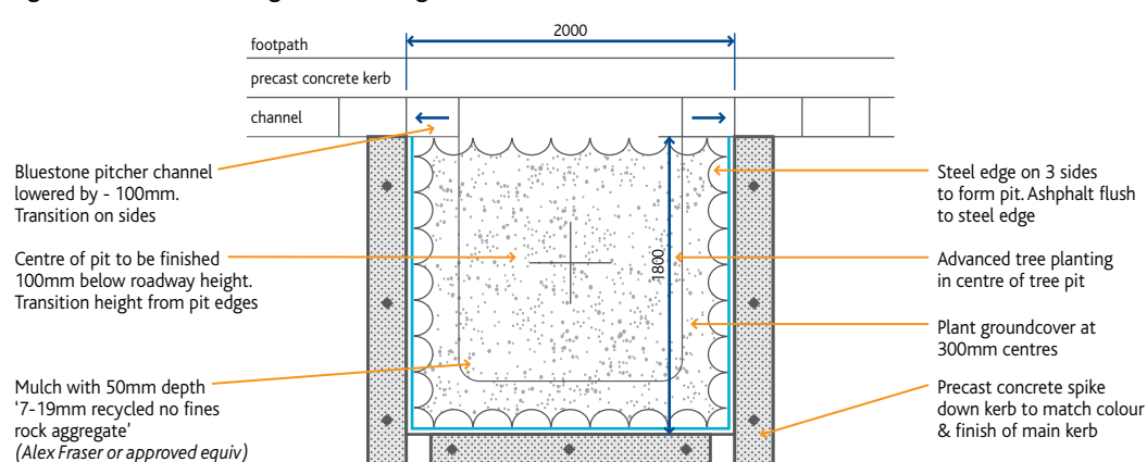
Figure 4. Plan view of raingarden showing surface details
