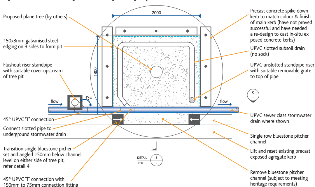
Figure 3. Plan view of raingarden showing drainage layout
