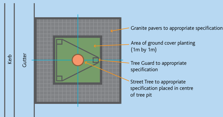
Figure 3. Raingarden tree pit integrated into the streetscape – situated roadside of kerb
