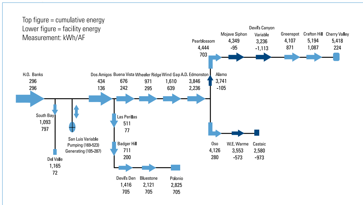
Figure 8. State Water Project Energy Inputs and Recovery. Robert Wilkinson, based on data from California Department of Water Resources. (kilowatt-hours per acre-foot pumped—including energy recovery)
