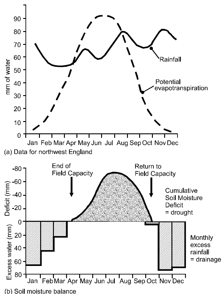
Figure 2.18 Typical average monthly moisture data
