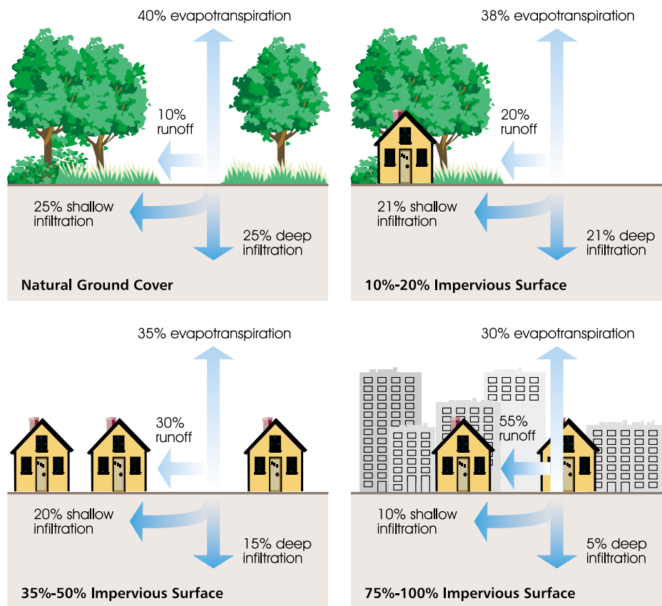
Figure 1.2. Runoff Variability with Increased Impervious Surfaces (FISWG, 1998)
