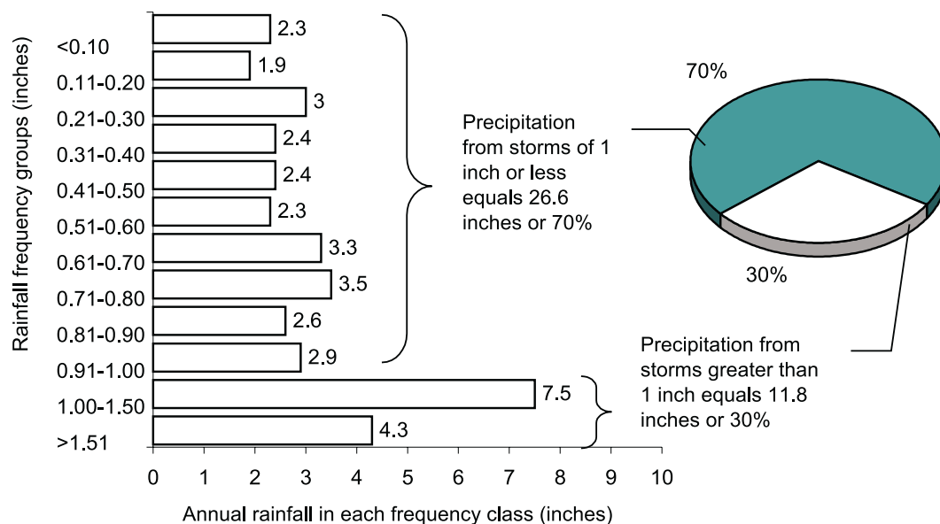
Figure 1.5. Rainfall Frequency Distribution at National Airport - 1980 to 1985
