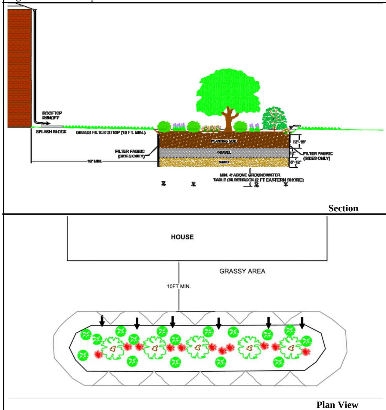
Figure 5.11 Landscape Infiltration
