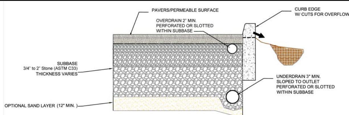
Typical Section w/Overdrain &amp; Underdrain
