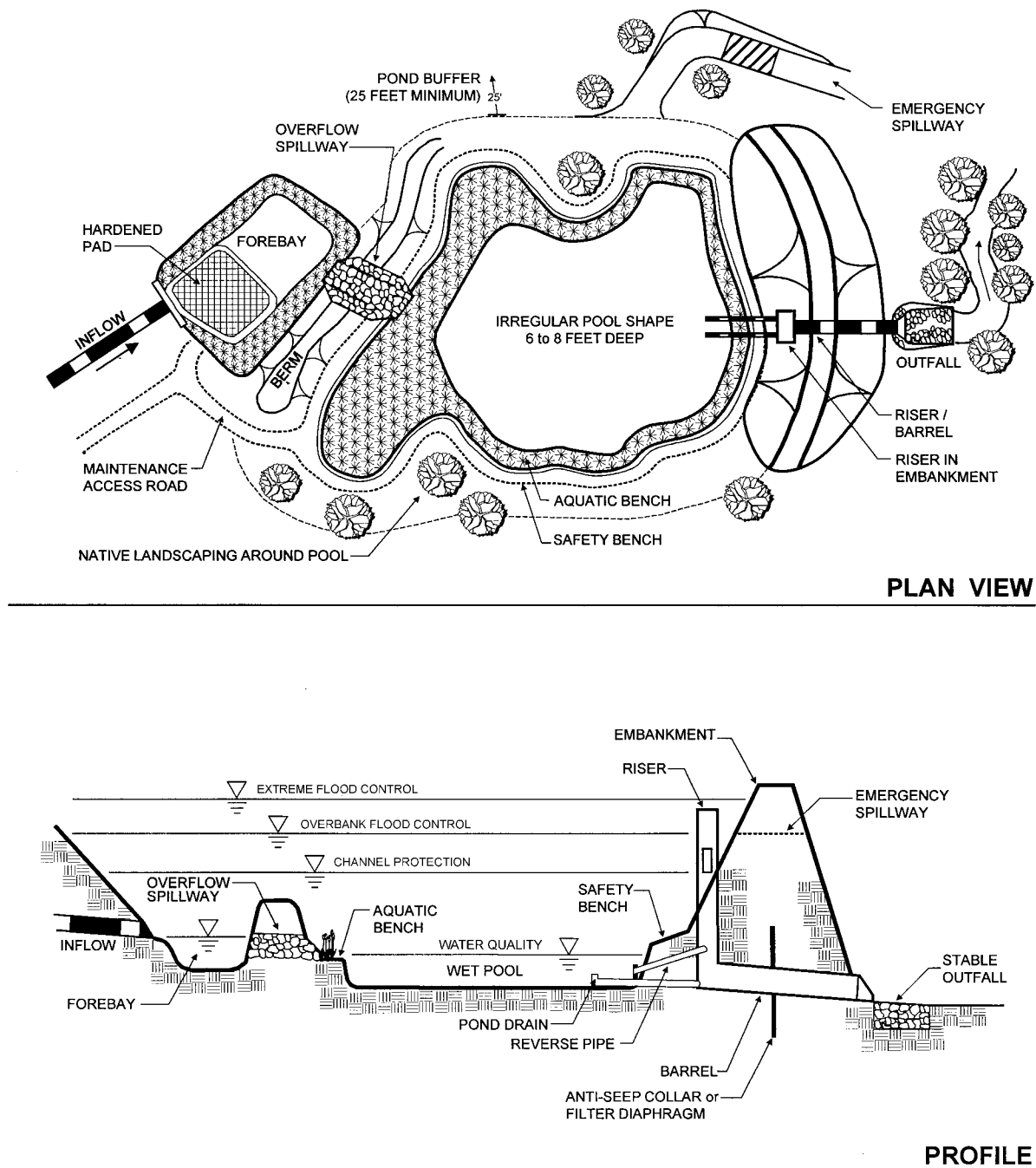
Figure 6.2 Wet Pond (P-2)
