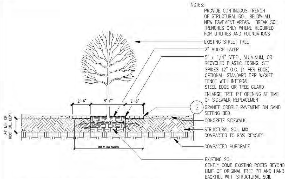
1A LONGITUDINAL SECTION TREE PIT
