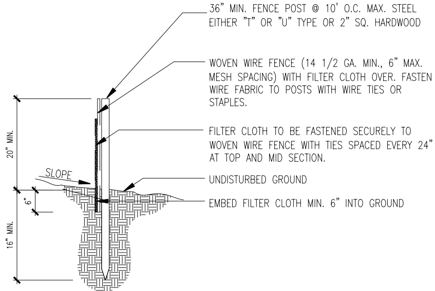
5 SILT FENCE NOT TO SCALE
