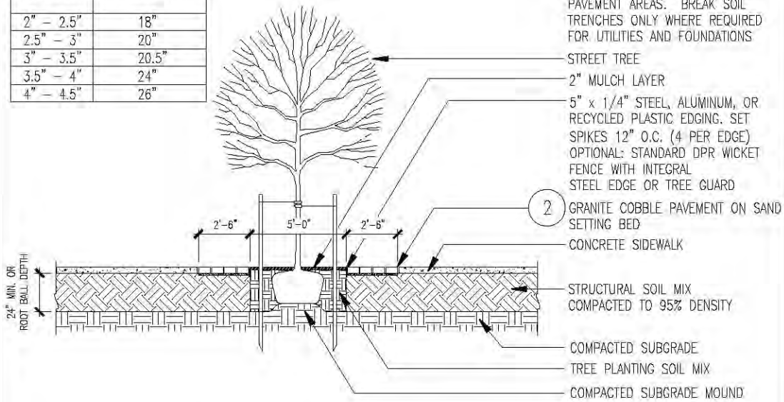
1 LONGITUDINAL SECTION TREE PIT
