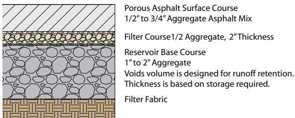
Porous asphalt pavement
