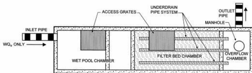
PLAN VIEW
