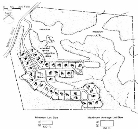
Figure 5.4-4 Hamlet or Village, (Source: Growing Greener: Putting Conservation Into Local Codes. Natural Lands Trust, Inc., 1997)
