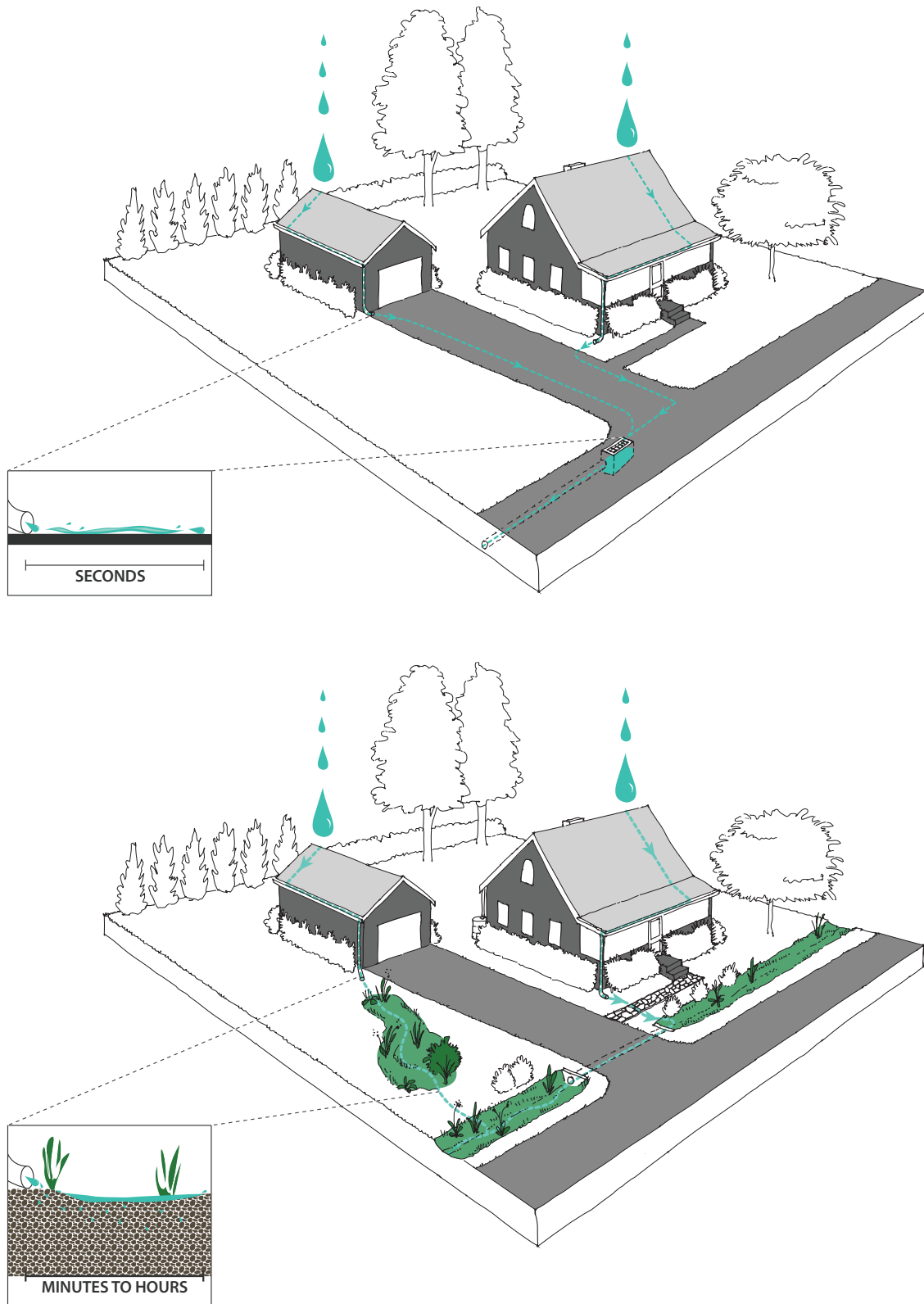
Figure 1-2 Designing to Increase Time of Concentration.
