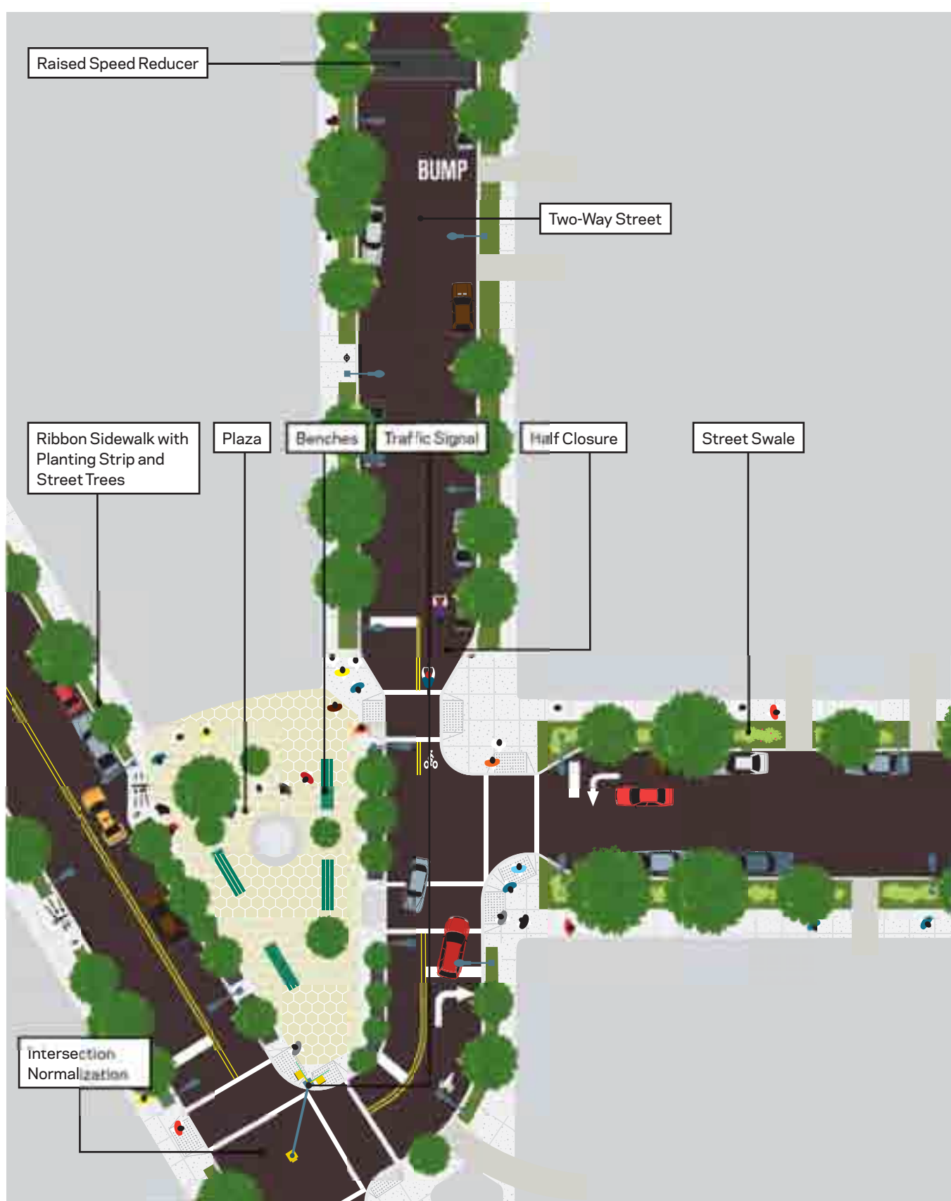
Figure 2 Treatments Appropriate to Local Streets
