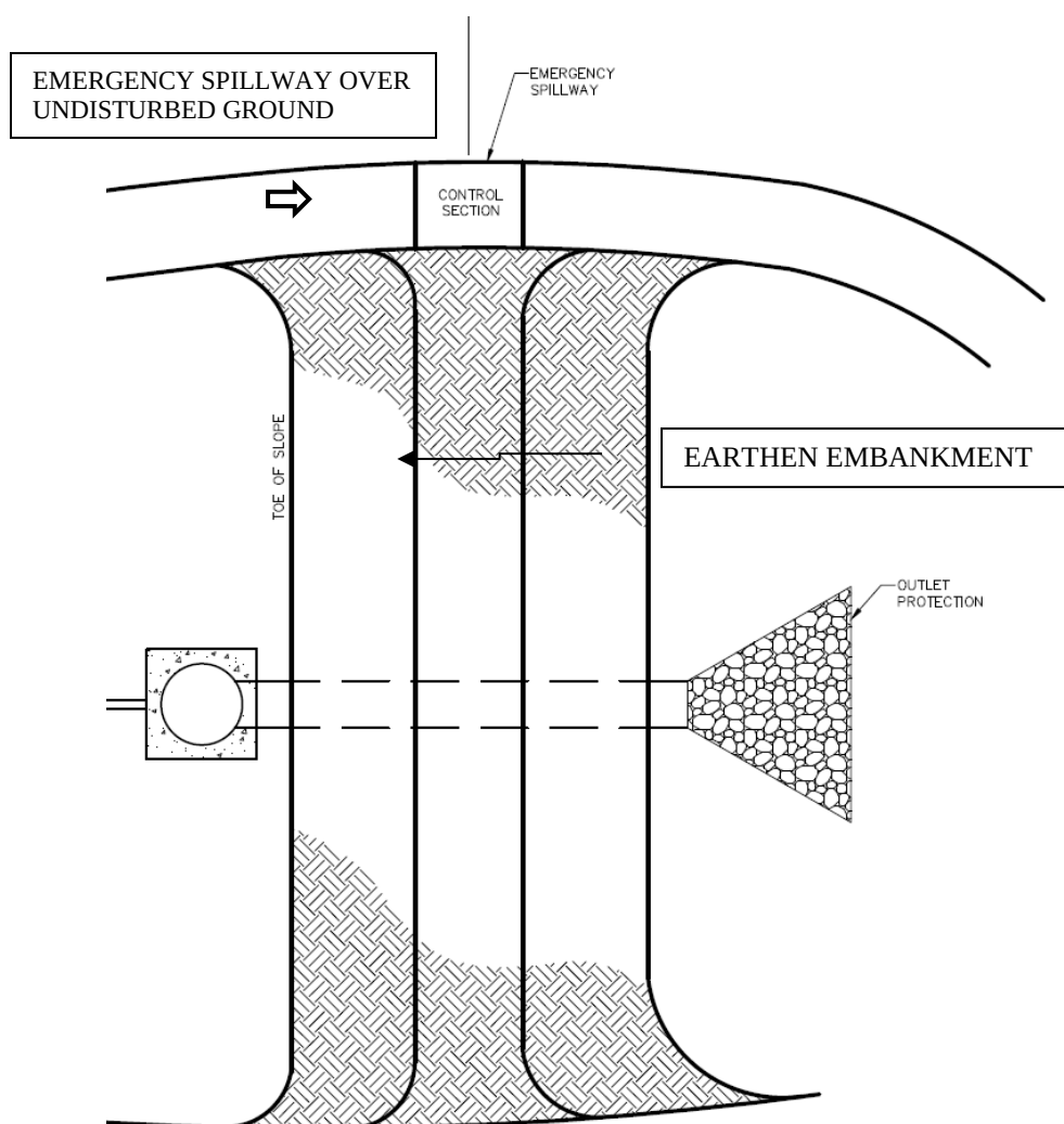
Figure 7.31-11 Earthen Embankment
