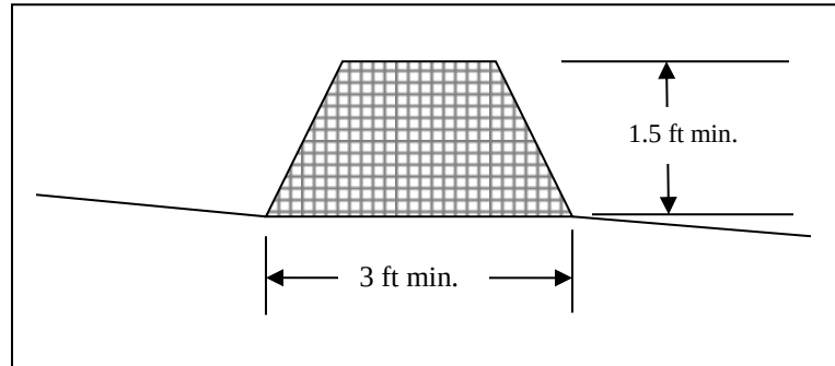
Figure 7.38-1 Filter Berm Dimensions
