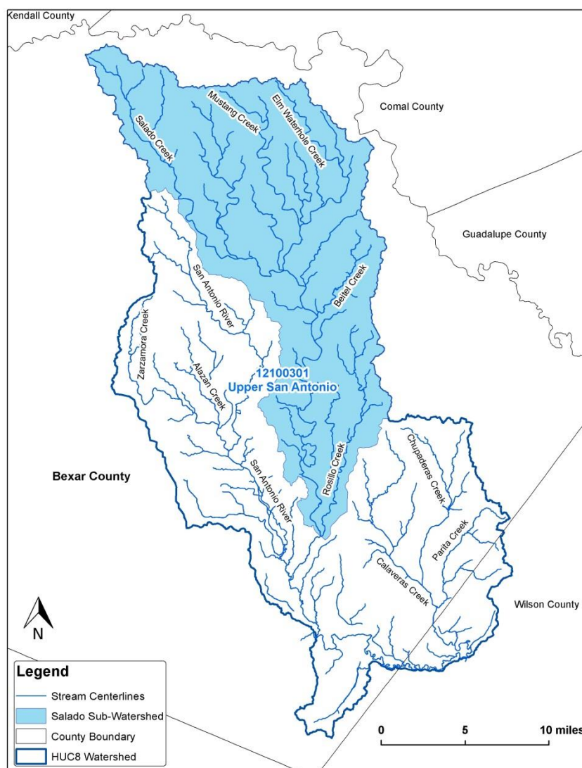
Figure 7–1. Streams in the Salado Creek subwatershed in relation to the Upper San Antonio HUC8.
