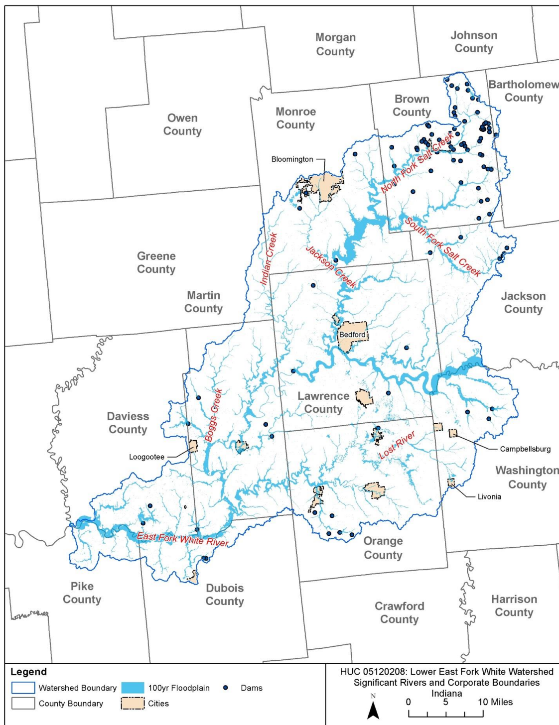
Figure B-10. HUC8 05120208, Lower East Fork White.
