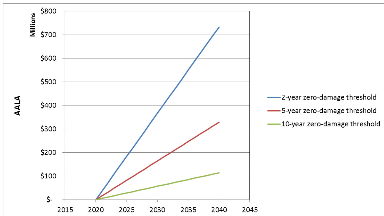
Figure 8–10. Assumed variation of the AALA in the conterminous United States between 2020 and 2040 (2011 dollars).
