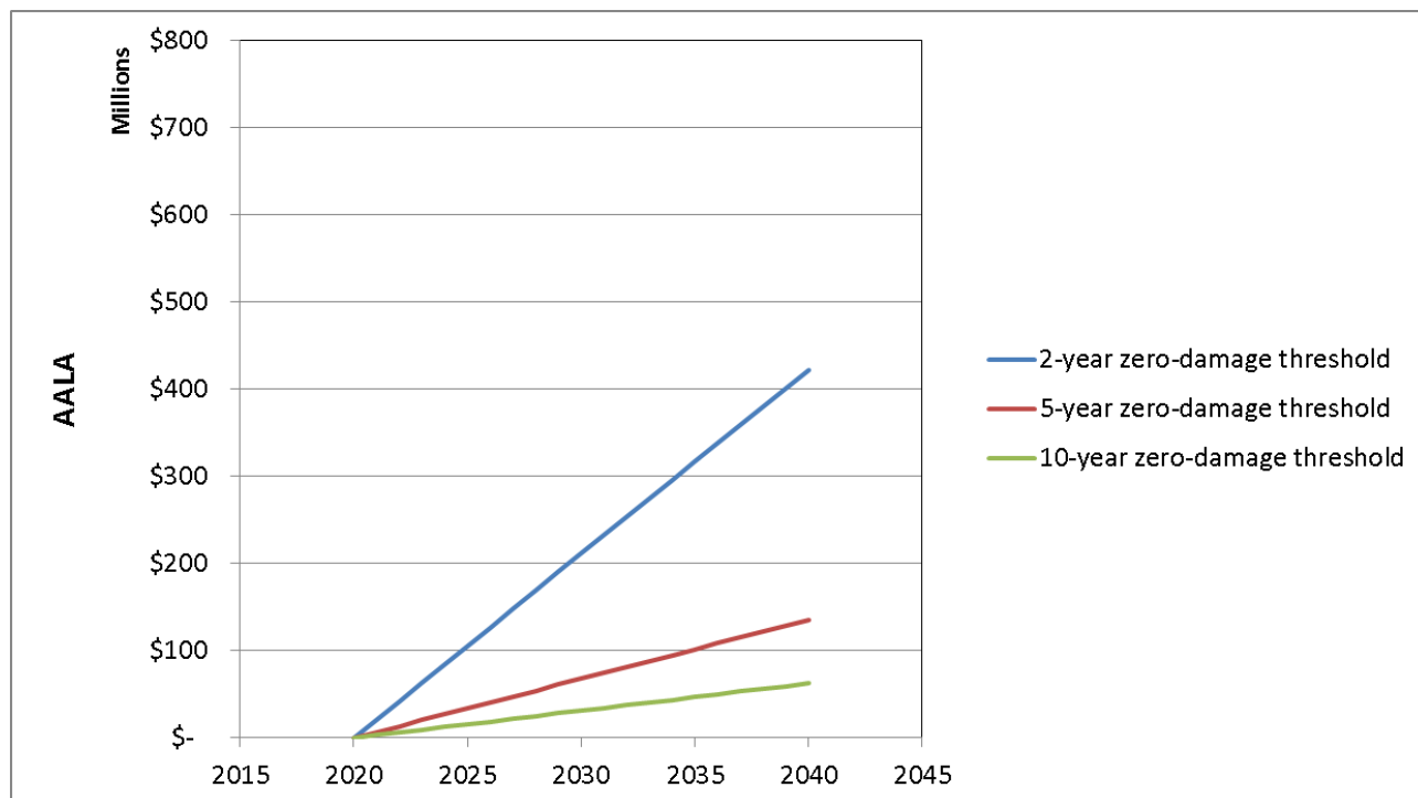
Figure 8–9. Assumed variation of the AALA in the conterminous United States between 2020 and 2040, excluding jurisdictions with GI-based retention standards (2011 dollars).
