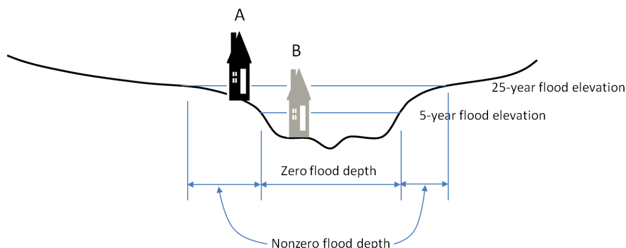
Figure 6–5. The uniform distribution in Hazus may place assets at risk in the 5- and the 25-year floodplains.
