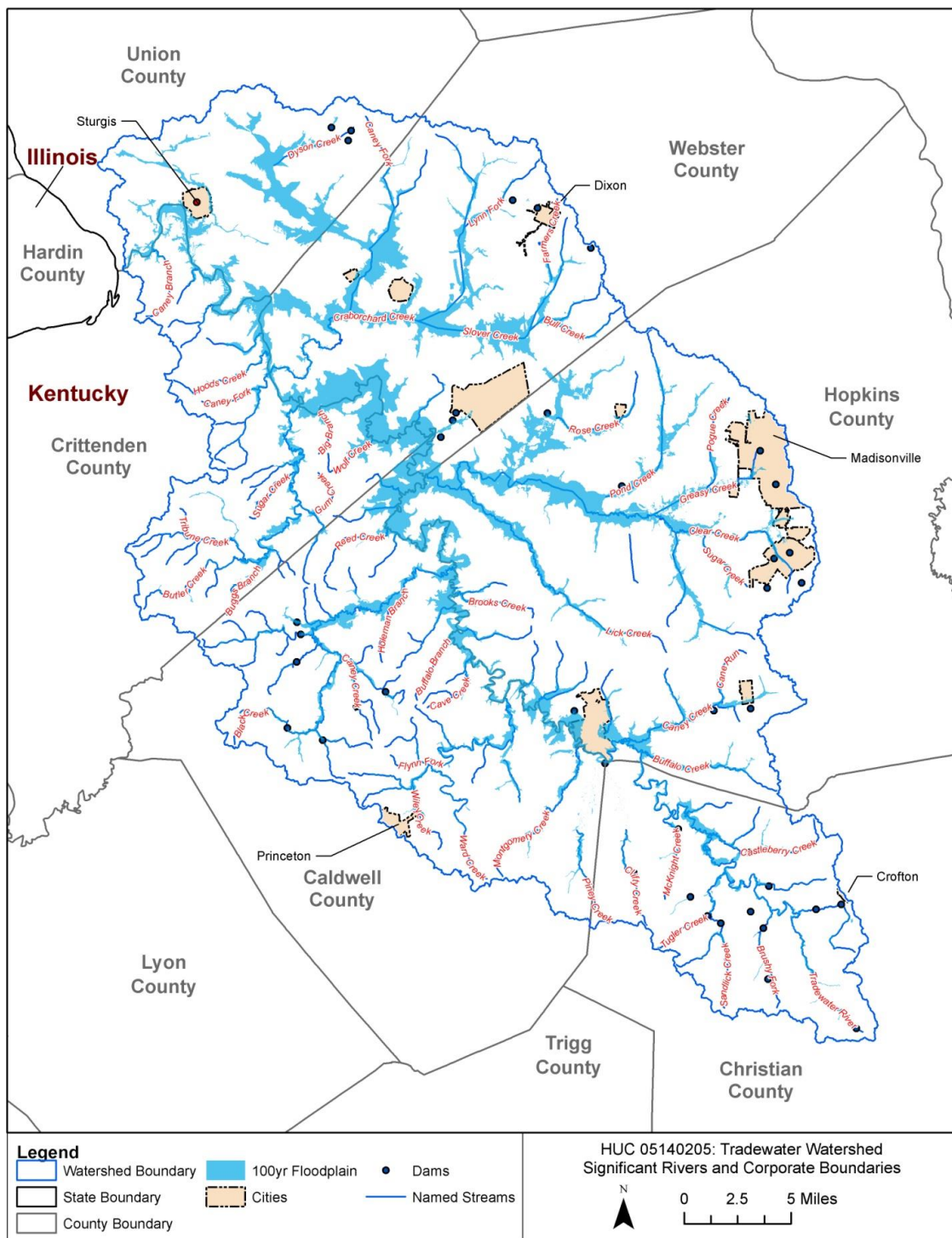
Figure B-11. HUC8 05140205, Tradewater.
