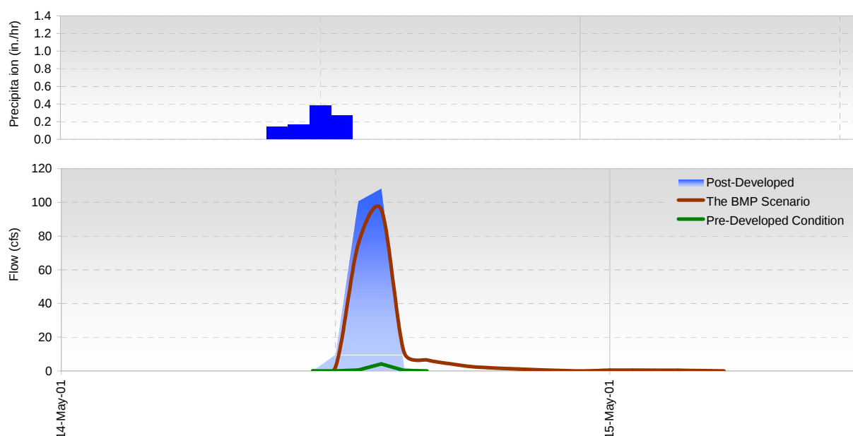
Figure 3-26. Storm event 2: May 14, 2001 11:00 a.m. to May 14, 2001 1:00 p.m. (0.95 in. to 4 wet hours, peak: 0.38 in.).
