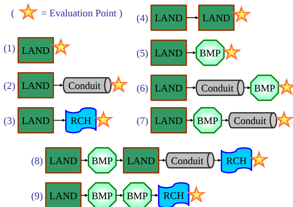
Figure A-1. Typical management configurations.
