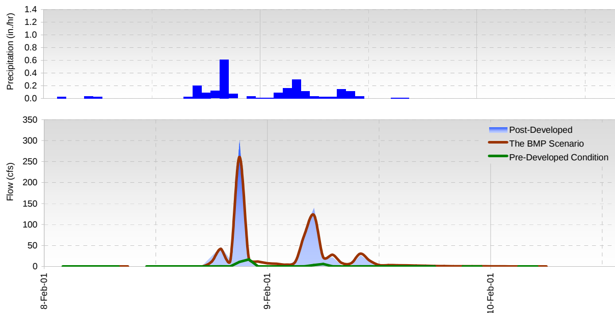
Figure 3-28. Storm event 4: February 8, 2001 12:00 a.m. to February 9, 2001 4:00 p.m. (2.34 in. to 25 wet hours, peak: 0.61 in.).
