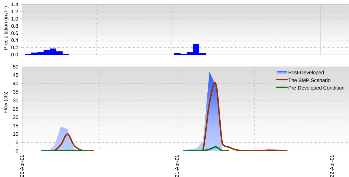
Figure 3-27. Storm event 3: April 20, 2001 2:00 a.m. to April 21, 2001 5:00 a.m. (1.03 in. to 12 wet hours, peak: 0.30 in.).
