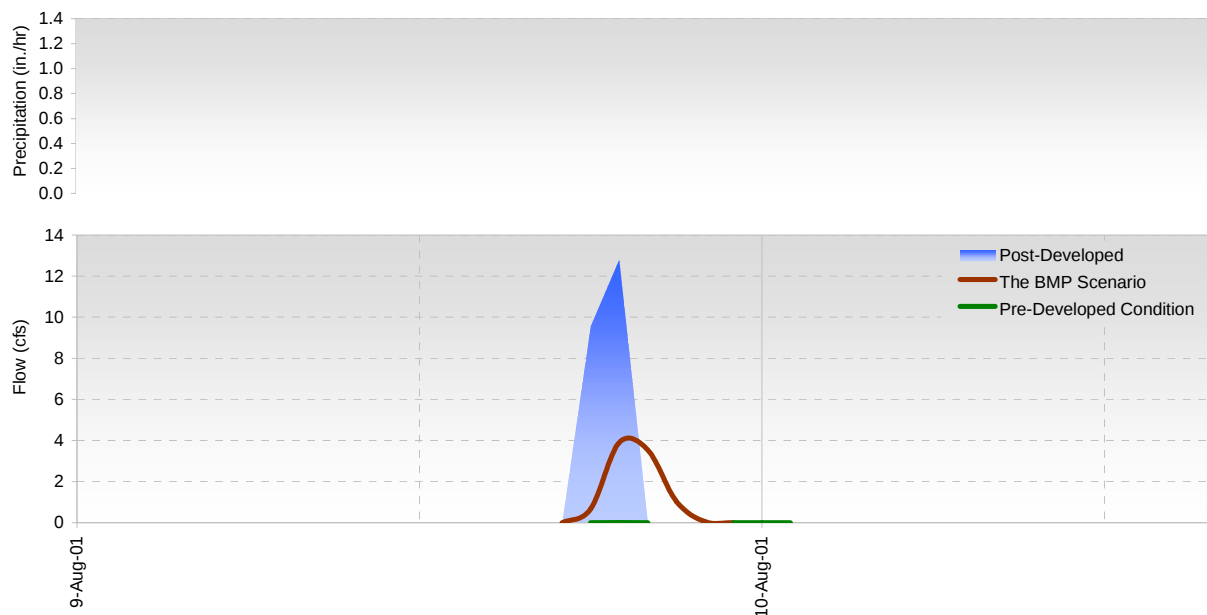
Figure 3-25. Storm event 1: August 9, 2001 6:00 p.m. to August 9, 2001 8:00 p.m. (0.66 in. to 2 wet hours, peak: 0.48 in.).
