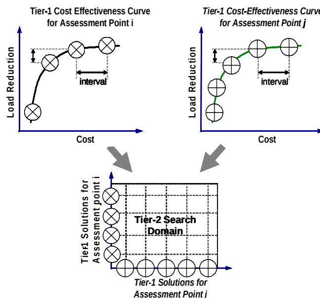
Figure 3-21. Construction of the tier-2 search domain using tier-1 results.
