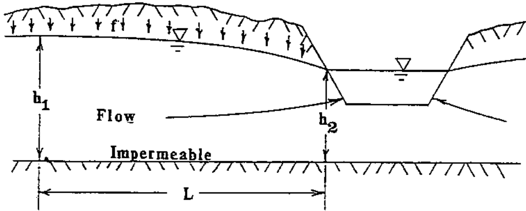
Figure 5-7 Definition sketch for Dupuit-Forcheimer seepage to an adjacent channel.
