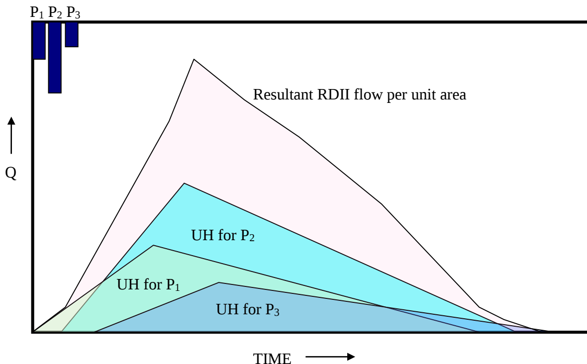
Figure 7-3 Application of a unit hydrograph to a storm event.
