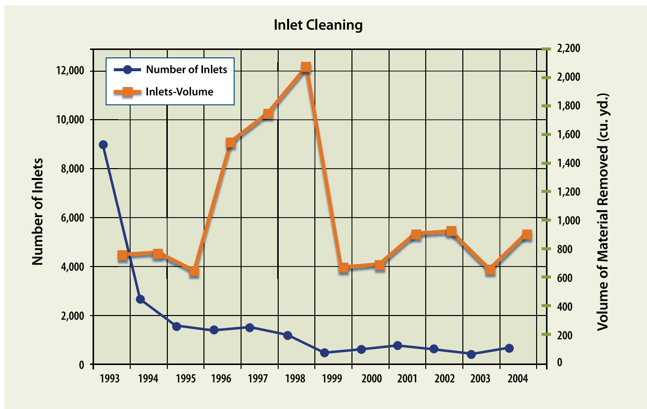
Figure 10.2. Inlet cleaning data derived from maintenance records
